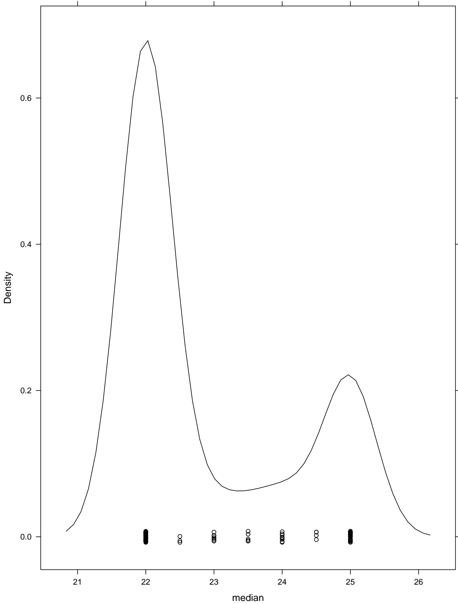
Density Plot
