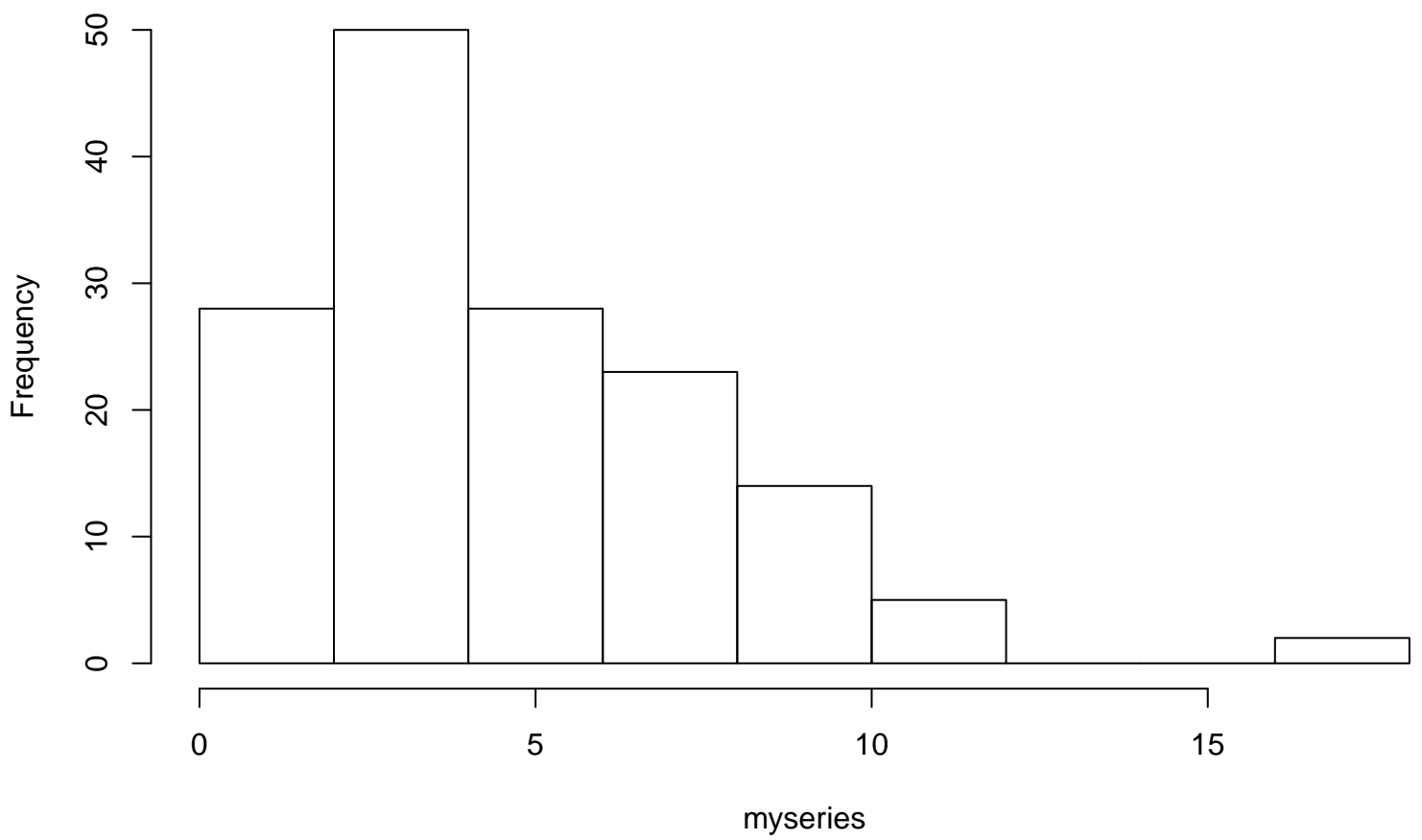
Histogram of myseries
