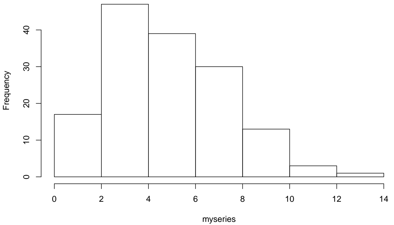
Histogram of myseries
