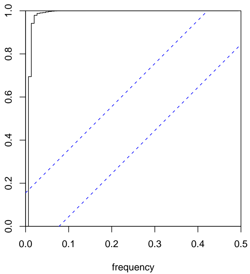
Cumulative Periodogram of myseries1 (d=0,D=0)
