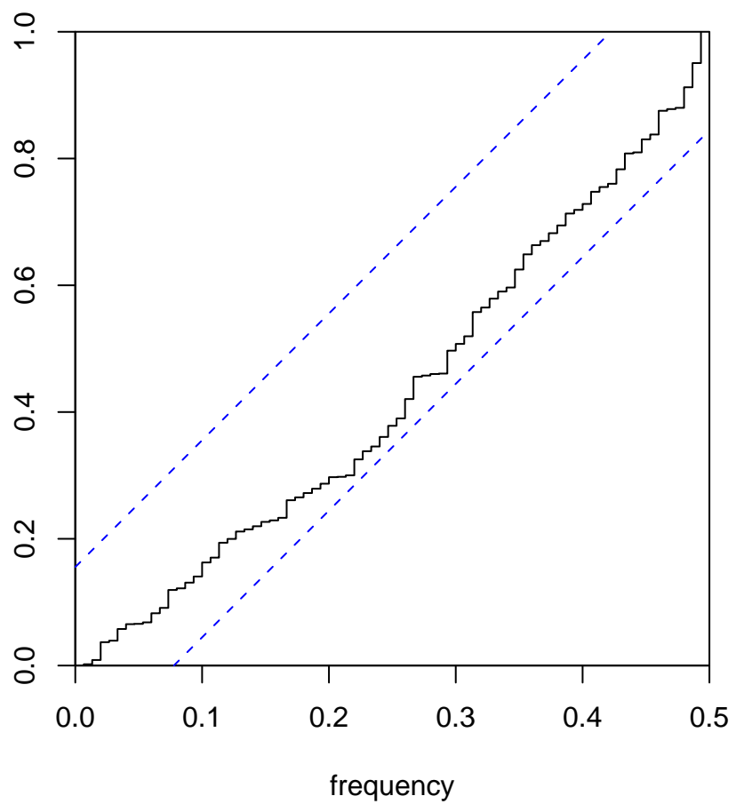
Cumulative Periodogram of myseries2 (d=0,D=0)
