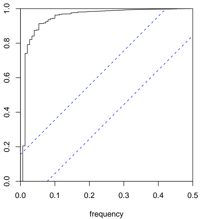
Cumulative Periodogram of myseries3 (d=0,D=0)
