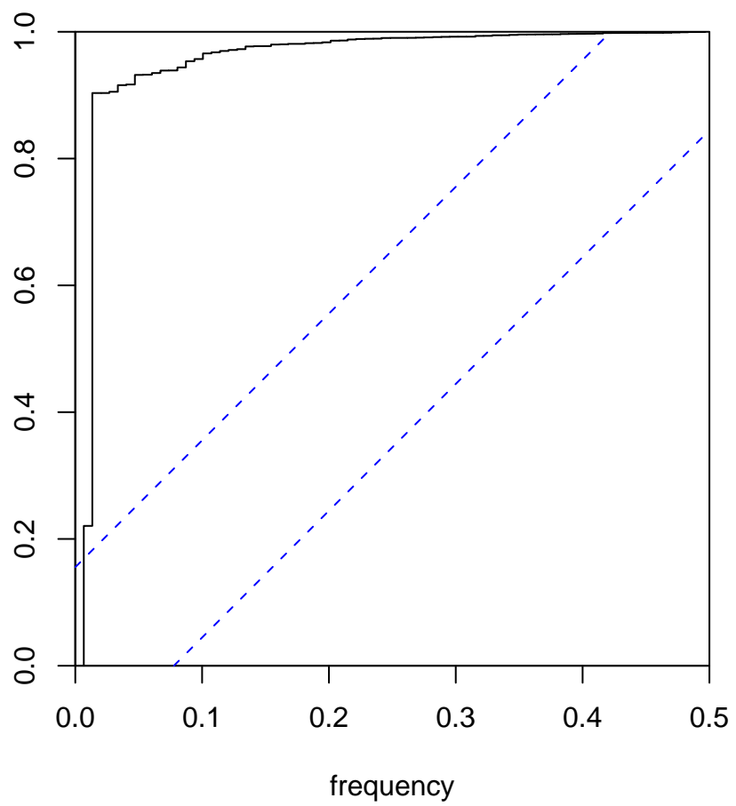
Cumulative Periodogram of myseries1 (d=1,D=0)
