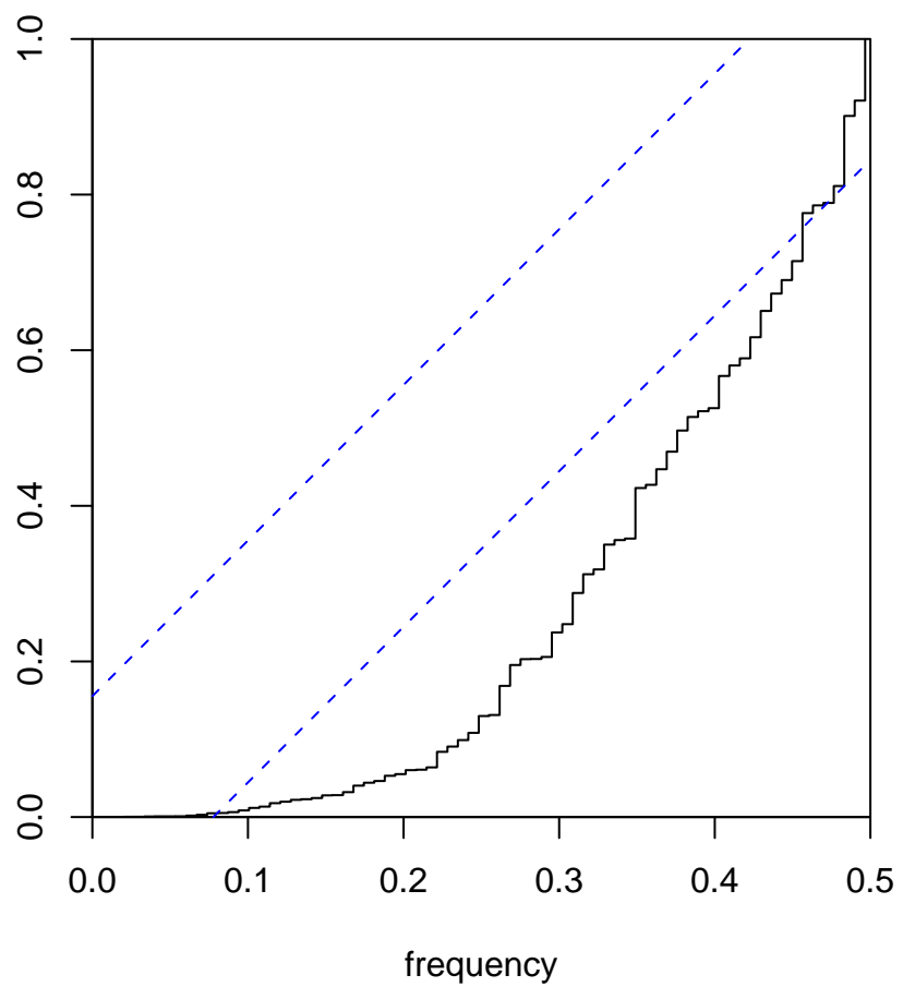
Cumulative Periodogram of myseries2 (d=1,D=0)
