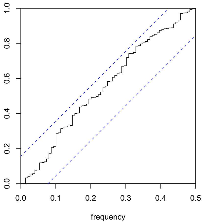
Cumulative Periodogram of myseries3 (d=1,D=0)
