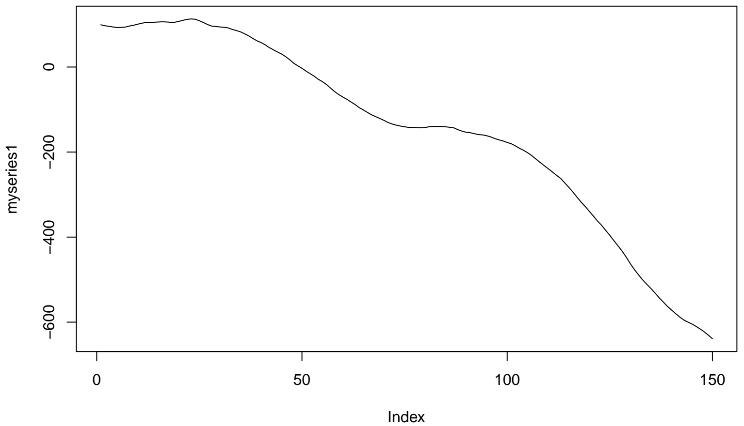
Run sequence plot of myseries1
