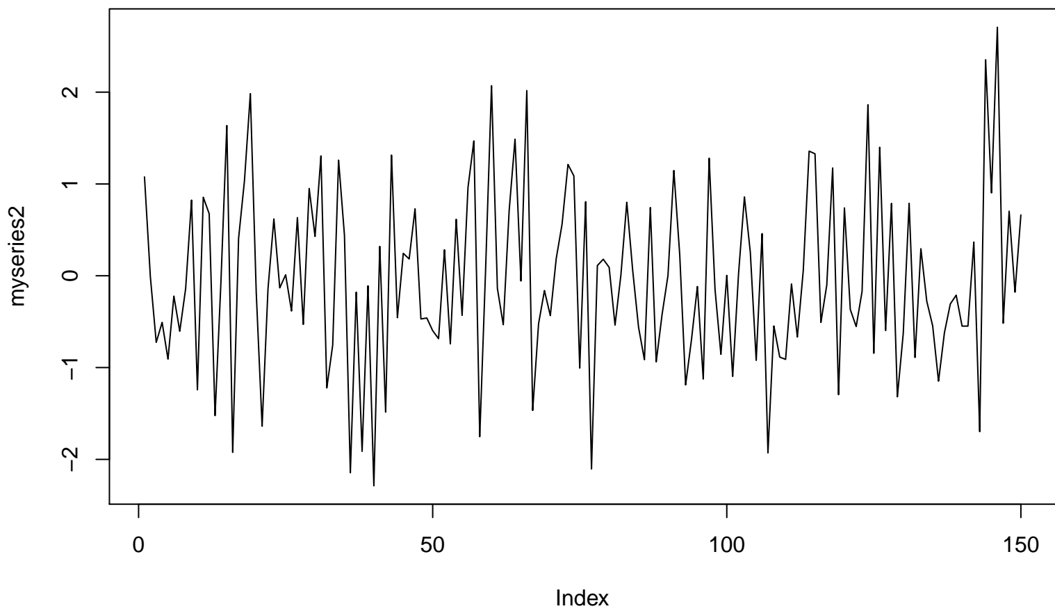
Run sequence plot of myseries2
