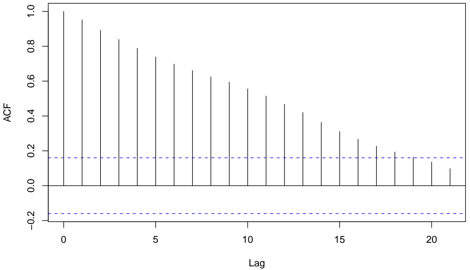
ACF of myseries3 (d=0,D=0)
