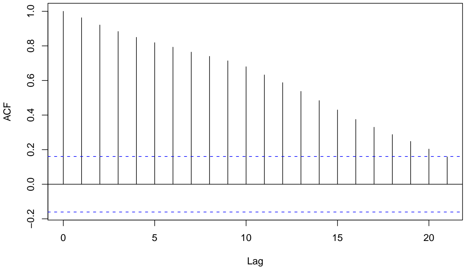
ACF of myseries1 (d=1,D=0)
