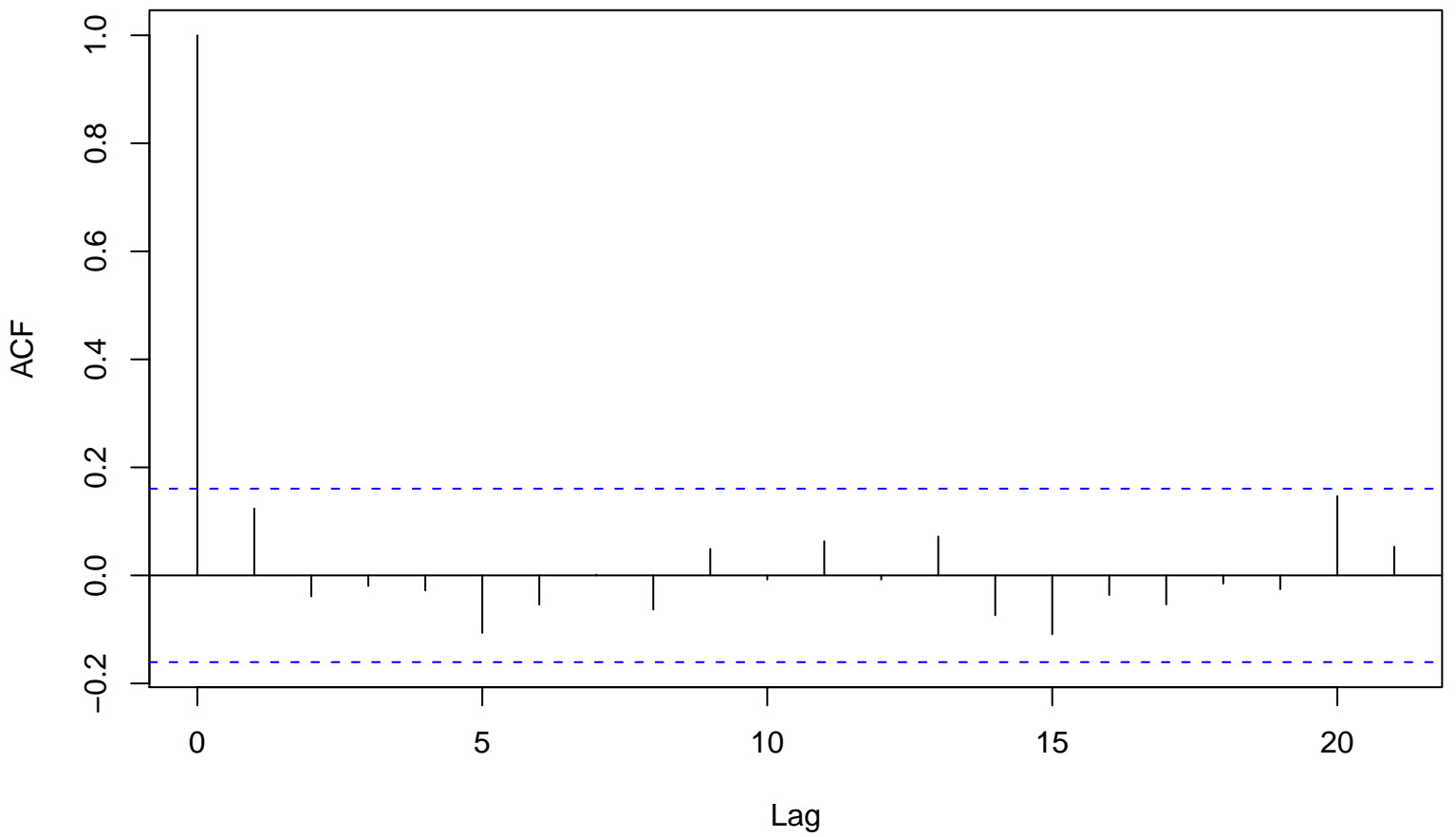
ACF of myseries3 (d=1,D=0)
