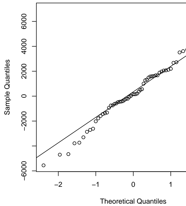
Residual Normal QQ Plot
