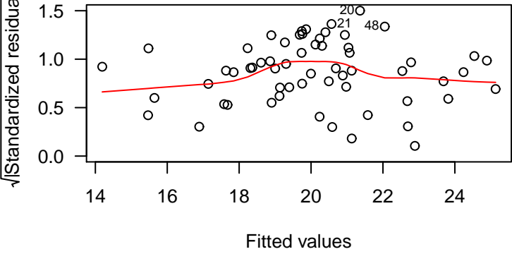
Scale-Location
