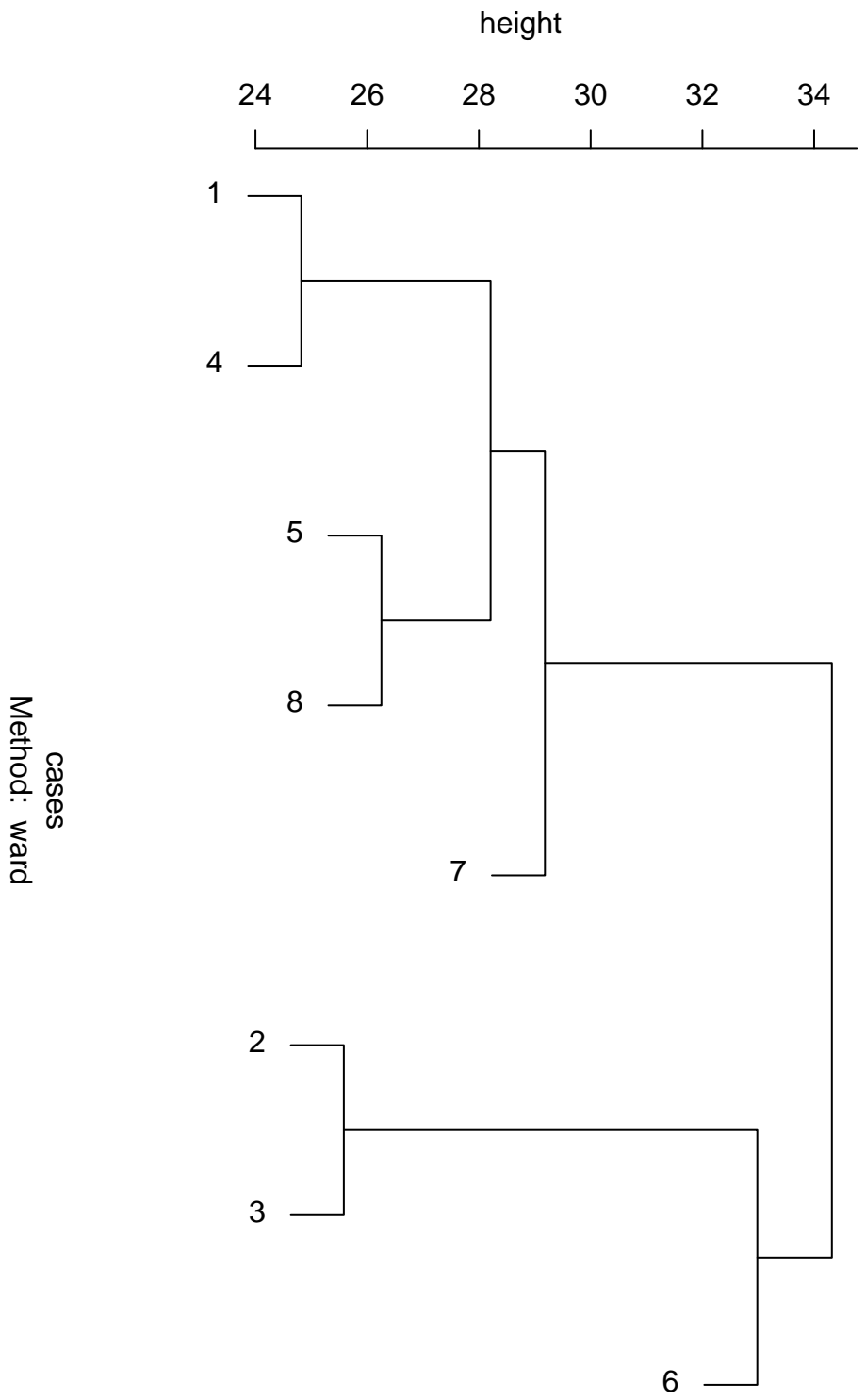
Dendrogram
