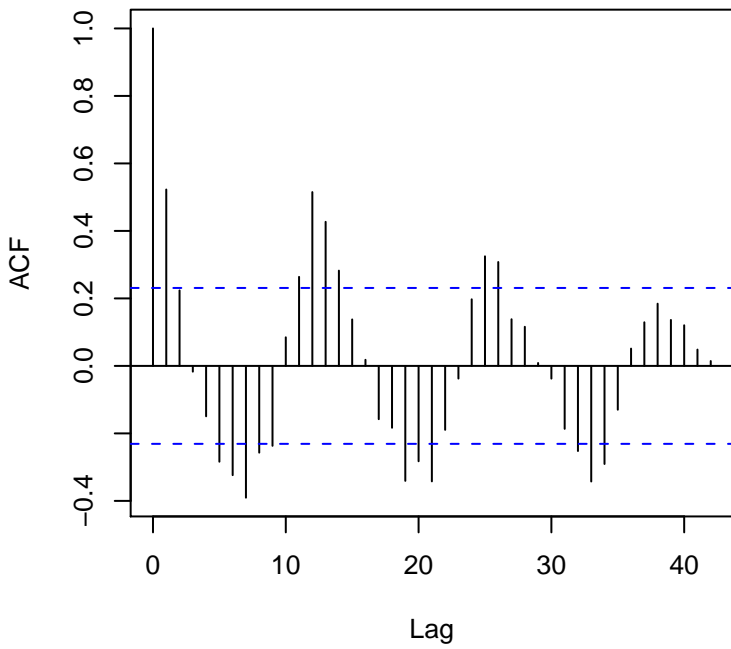
Residual ACF
