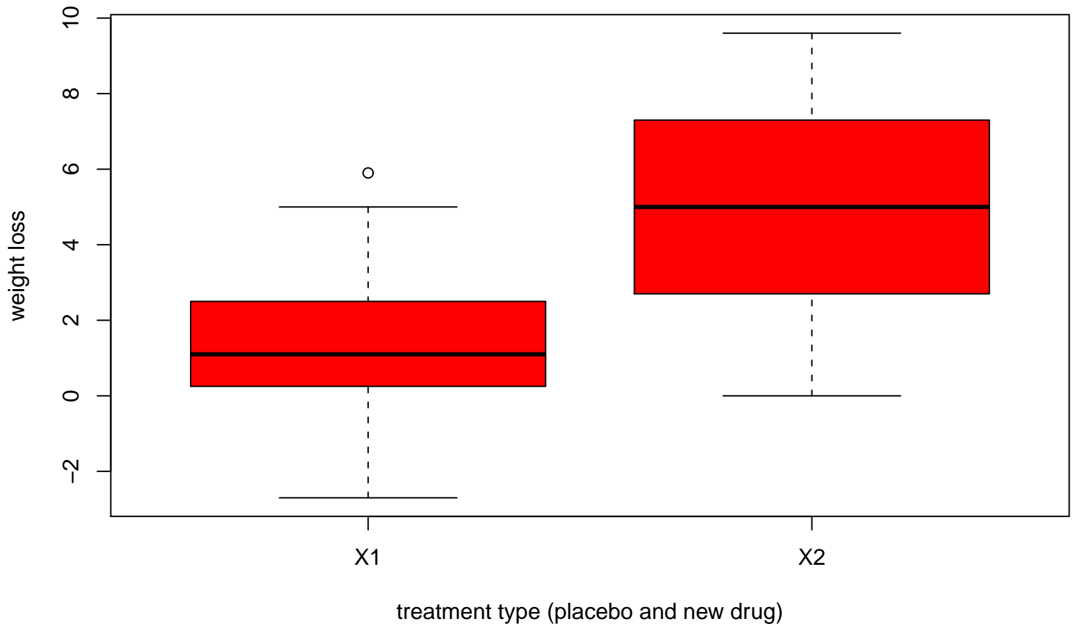
Boxplots Title
