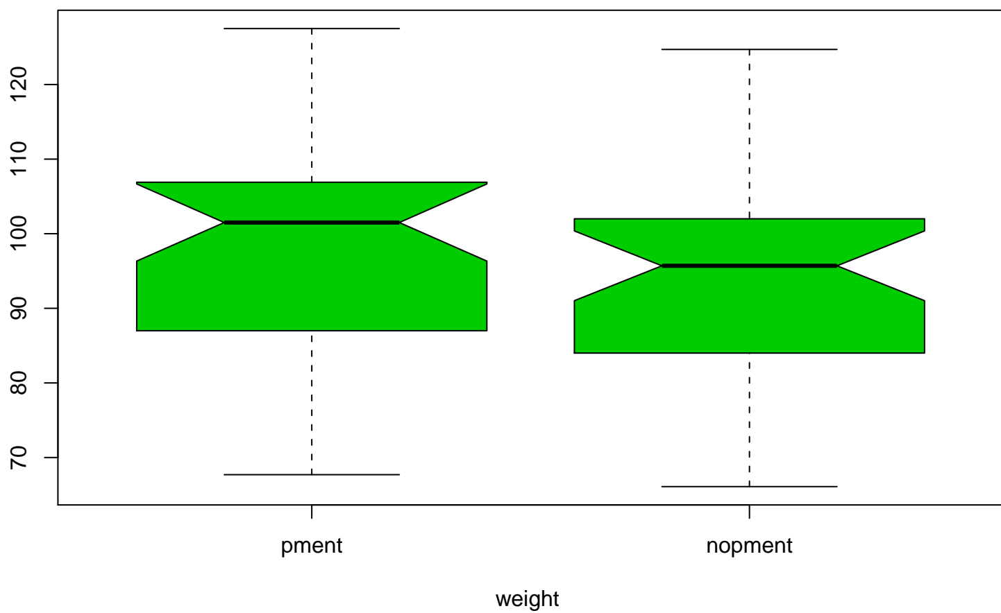
box plot
