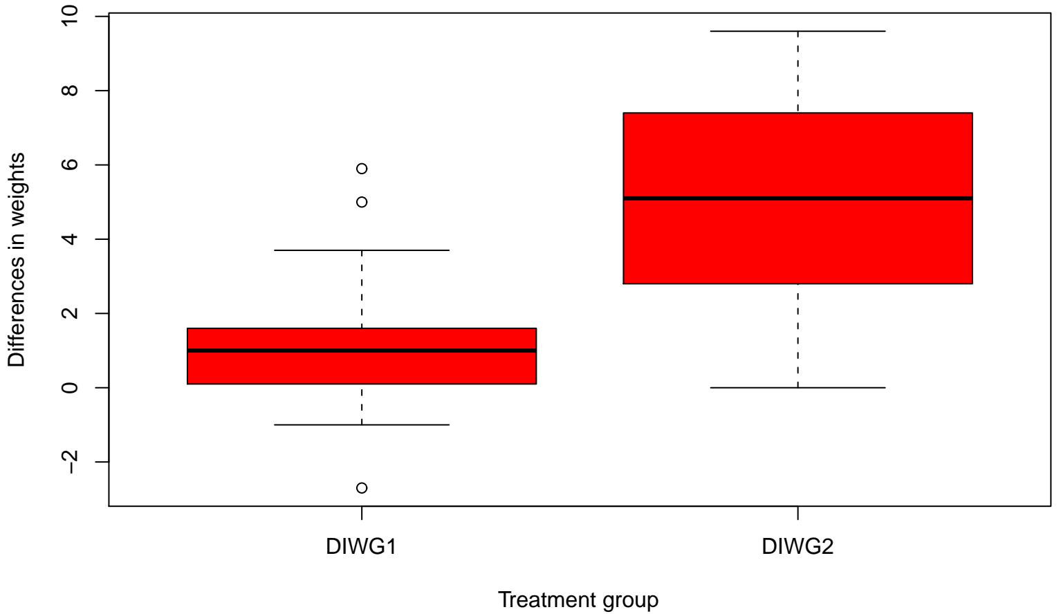
Boxplot showing differences in weights
