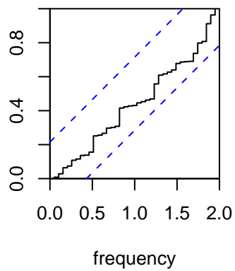
Residual Cumulative Periodogram
