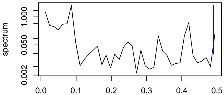
frequency bandwidth = 0.00356
