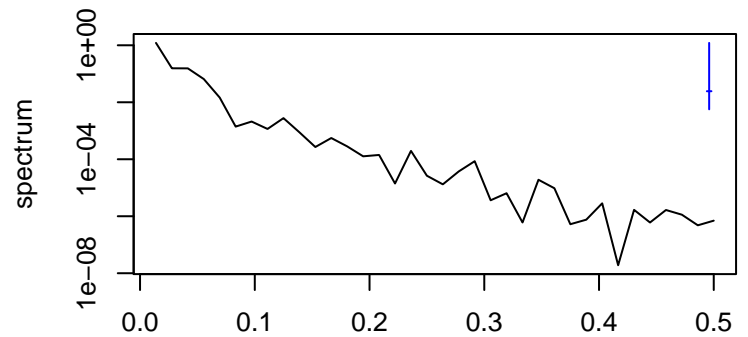
frequency bandwidth = 0.00401
