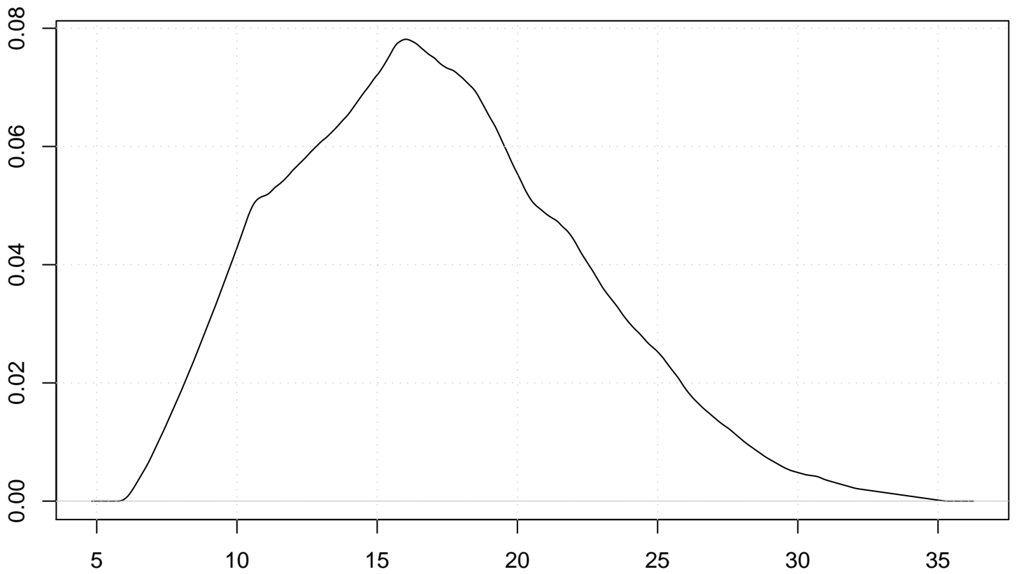
Triangular Kernel
