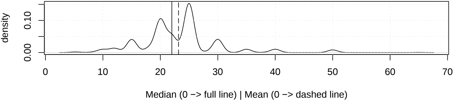
Density Plot – Gaussian Kernel
