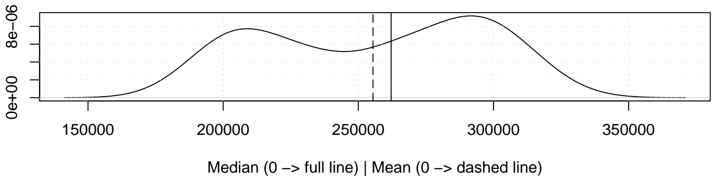
Density Plot – Gaussian Kernel
