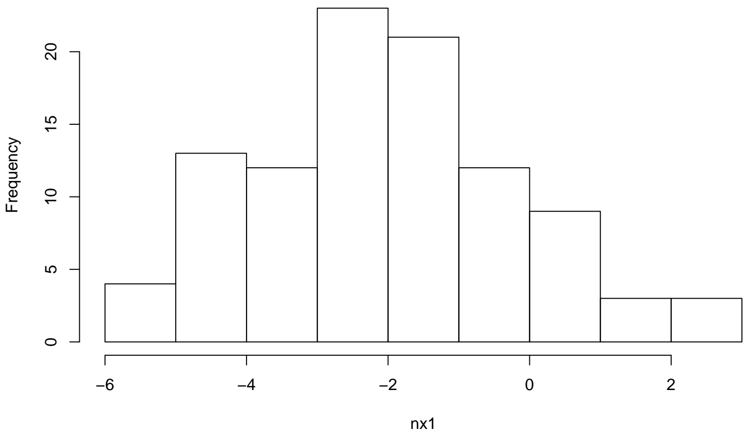
Histogram of nx1
