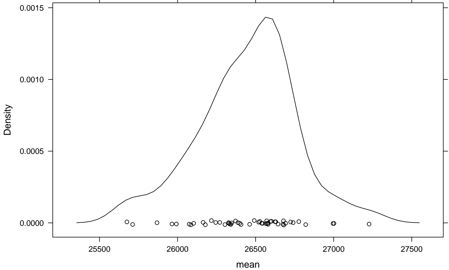
Density Plot
