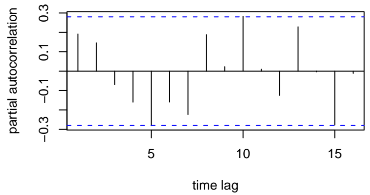
Residual PACF
