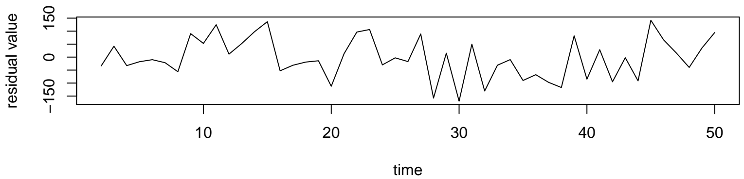
Residuals
