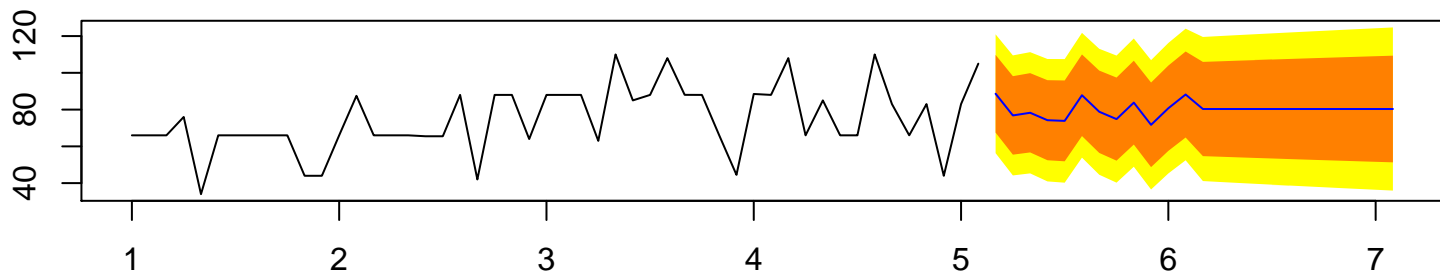
Forecasts from ARIMA(0,1,1)(0,0,1)[12]
