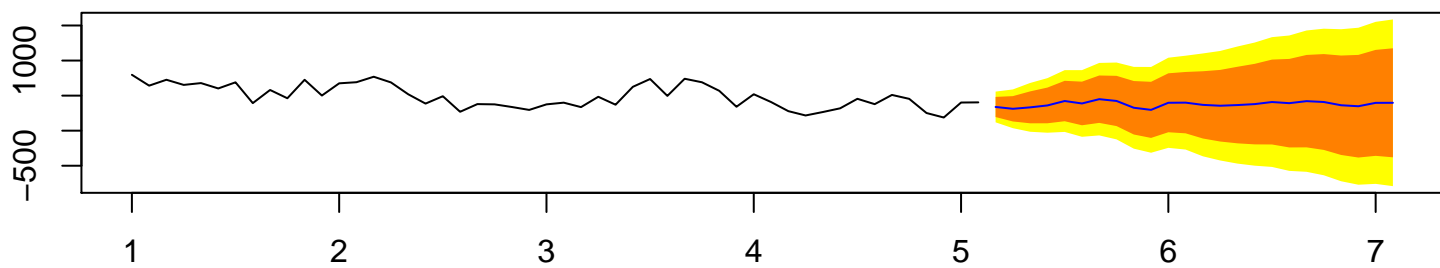
Forecasts from ARIMA(1,1,1)(1,0,0)[12]
