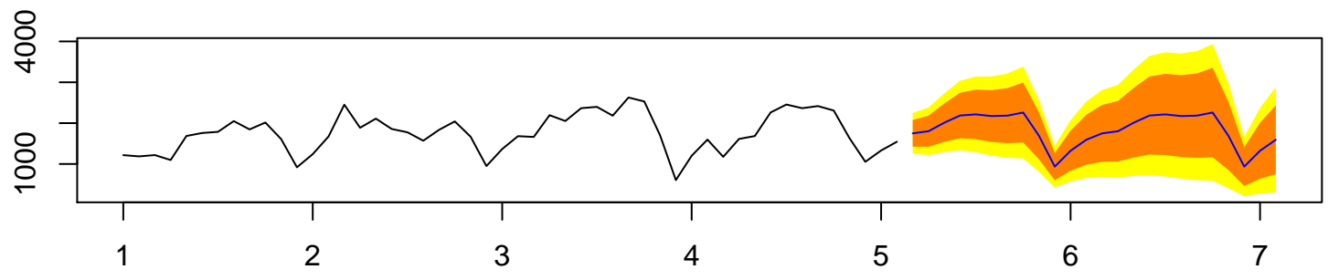
Forecasts from ETS(M,N,M)
