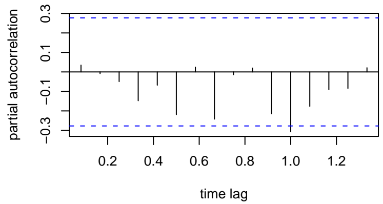
Residual PACF
