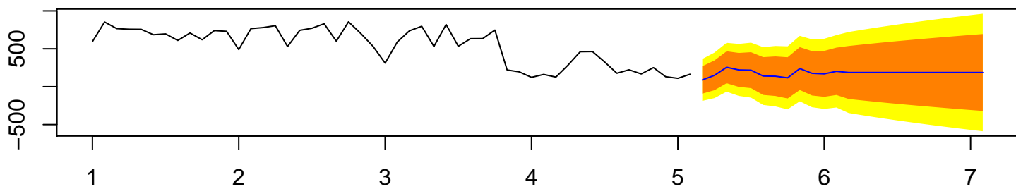
Forecasts from ARIMA(0,1,1)(0,0,1)[12]
