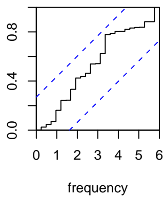
Cumulative Periodogram of Residuals
