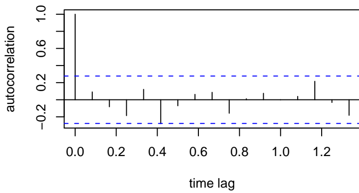
Residual ACF
