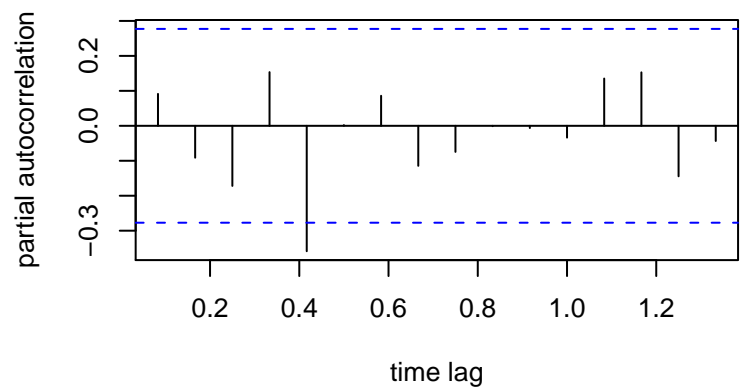
Residual PACF
