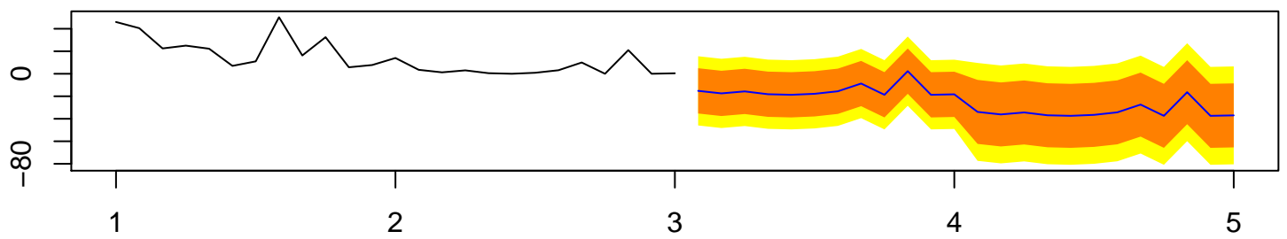
Forecasts from ARIMA(0,0,0)(0,1,0)[12] with drift
