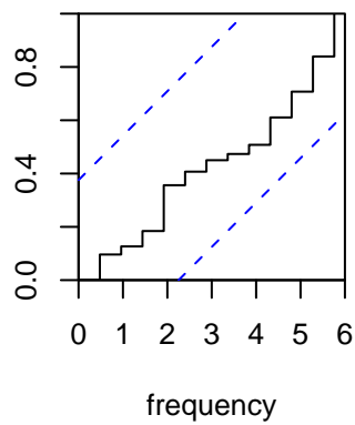
Cumulative Periodogram of Residuals
