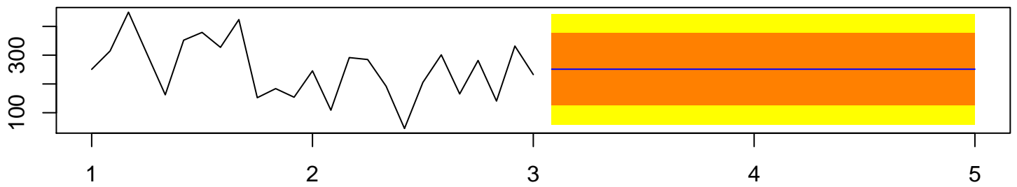
Forecasts from ARIMA(0,0,0) with non-zero mean
