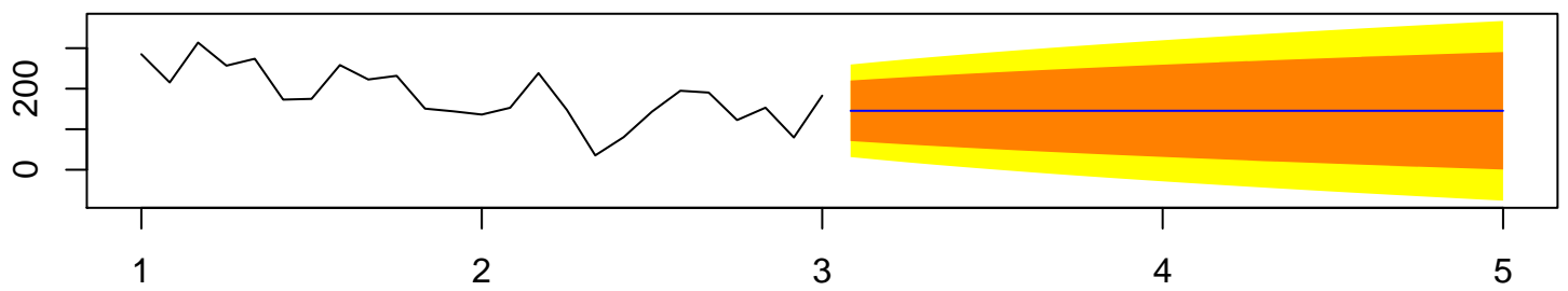
Forecasts from ARIMA(0,1,1)
