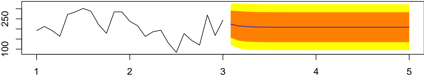
Forecasts from ARIMA(1,0,0) with non-zero mean
