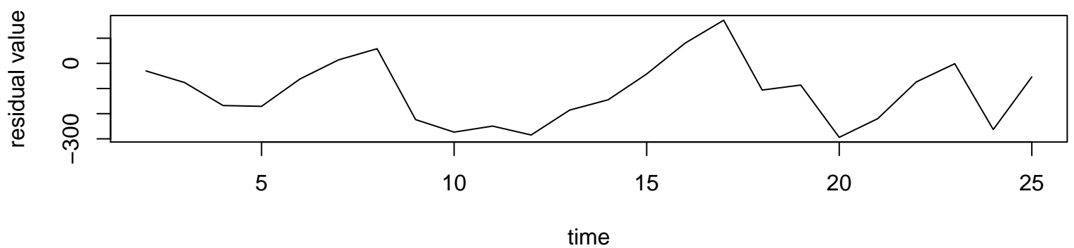
Residuals
