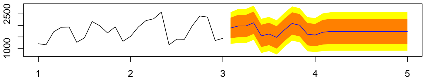
Forecasts from ARIMA(0,0,1)(0,0,1)[12] with non-zero mean
