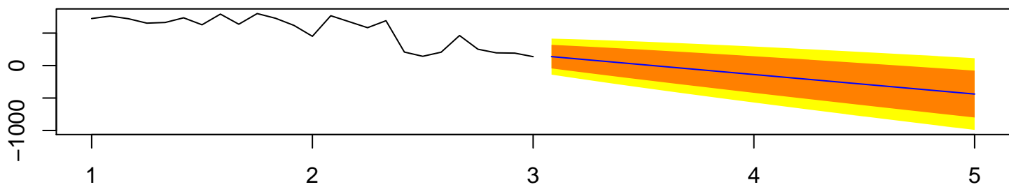
Forecasts from ARIMA(0,1,1) with drift
