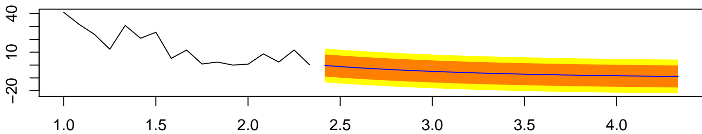
Forecasts from ETS(A,Ad,N)
