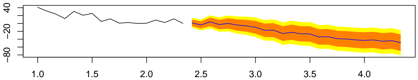
Forecasts from ARIMA(1,1,0)(1,0,0)[12] with drift
