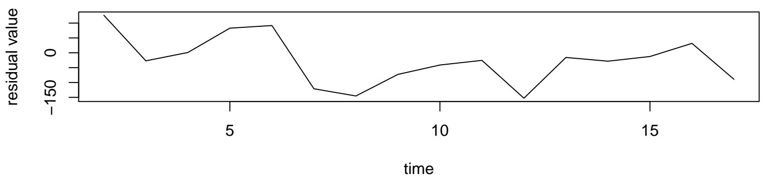
Residuals
