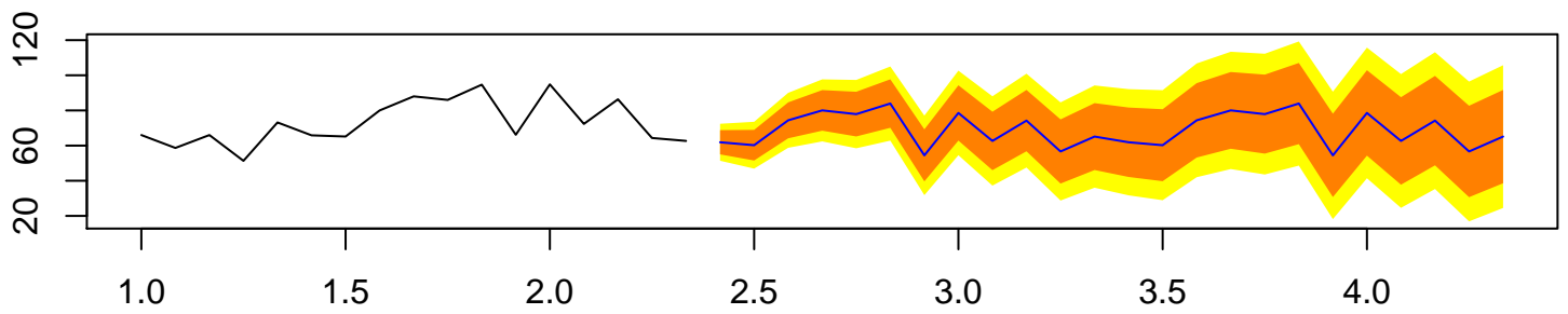
Forecasts from ETS(A,N,A)
