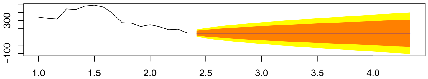
Forecasts from ETS(M,N,N)
