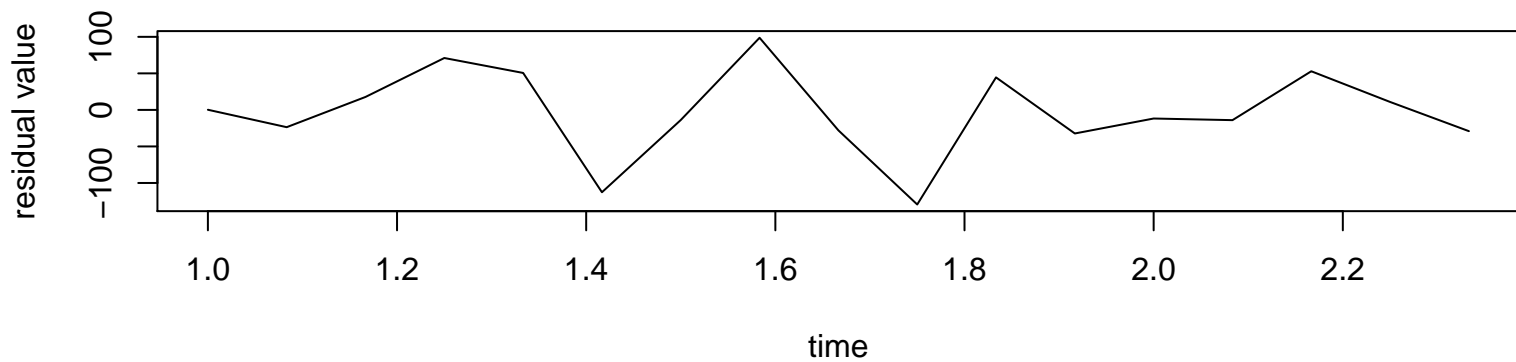
Residuals
