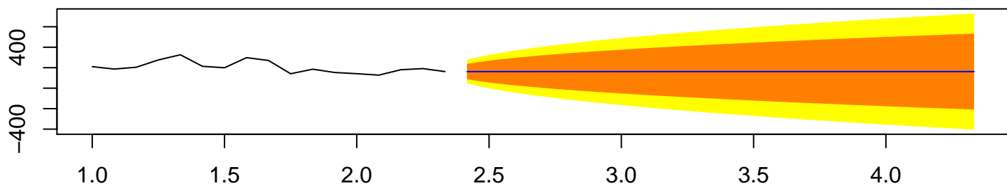
Forecasts from ARIMA(0,1,0)
